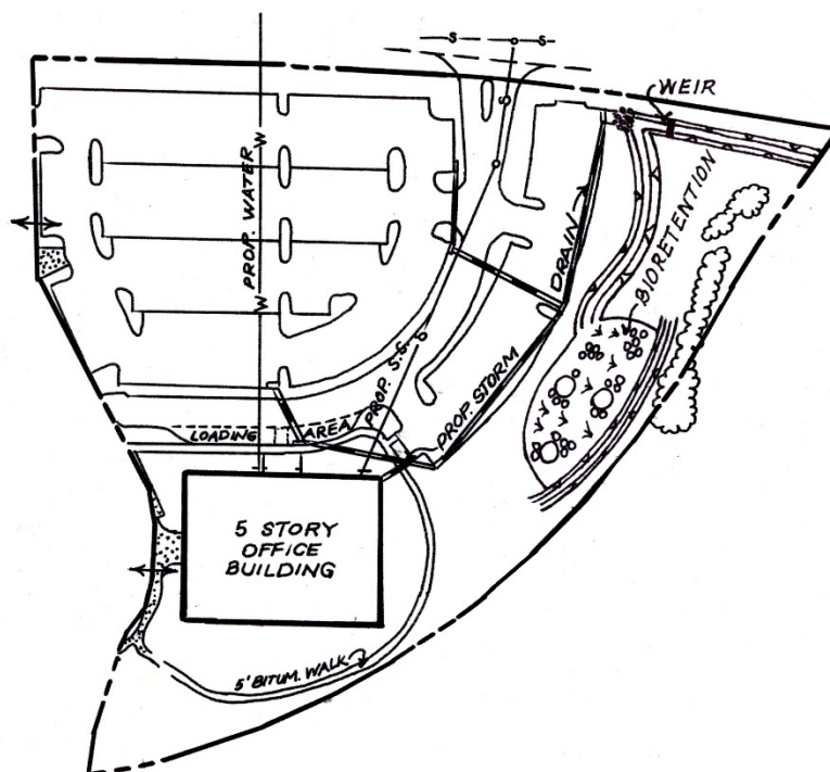
Figure 8.20 Lake Center Site Plan
