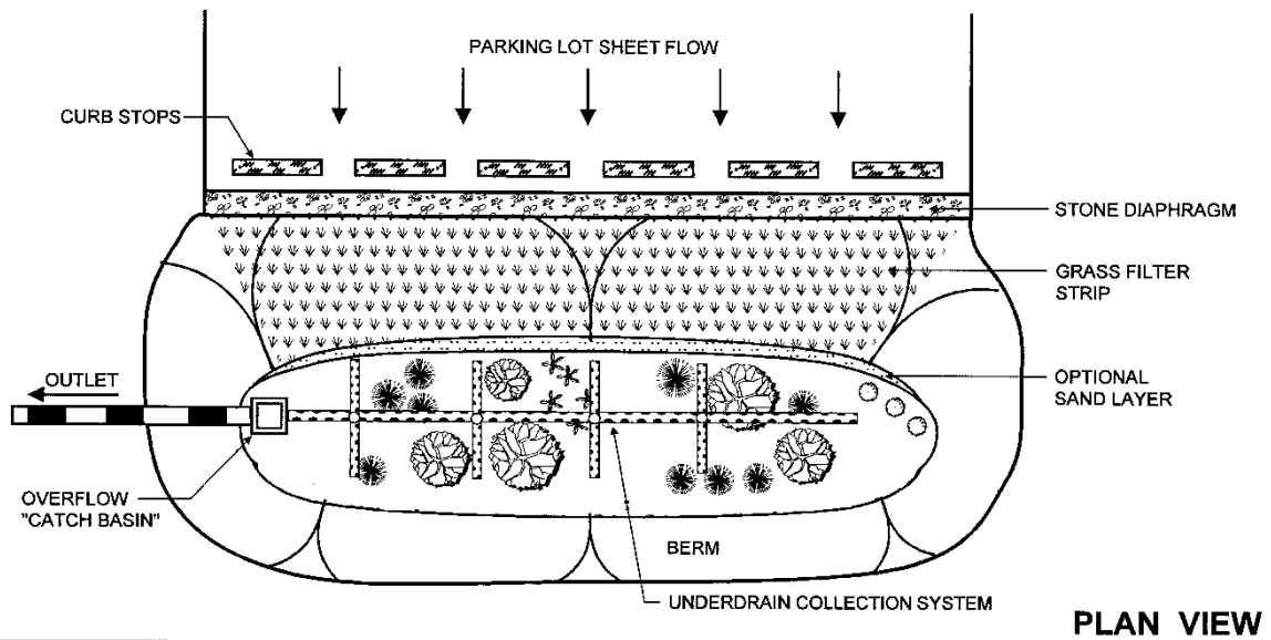
Figure 6.19 Bioretention (F-5)
