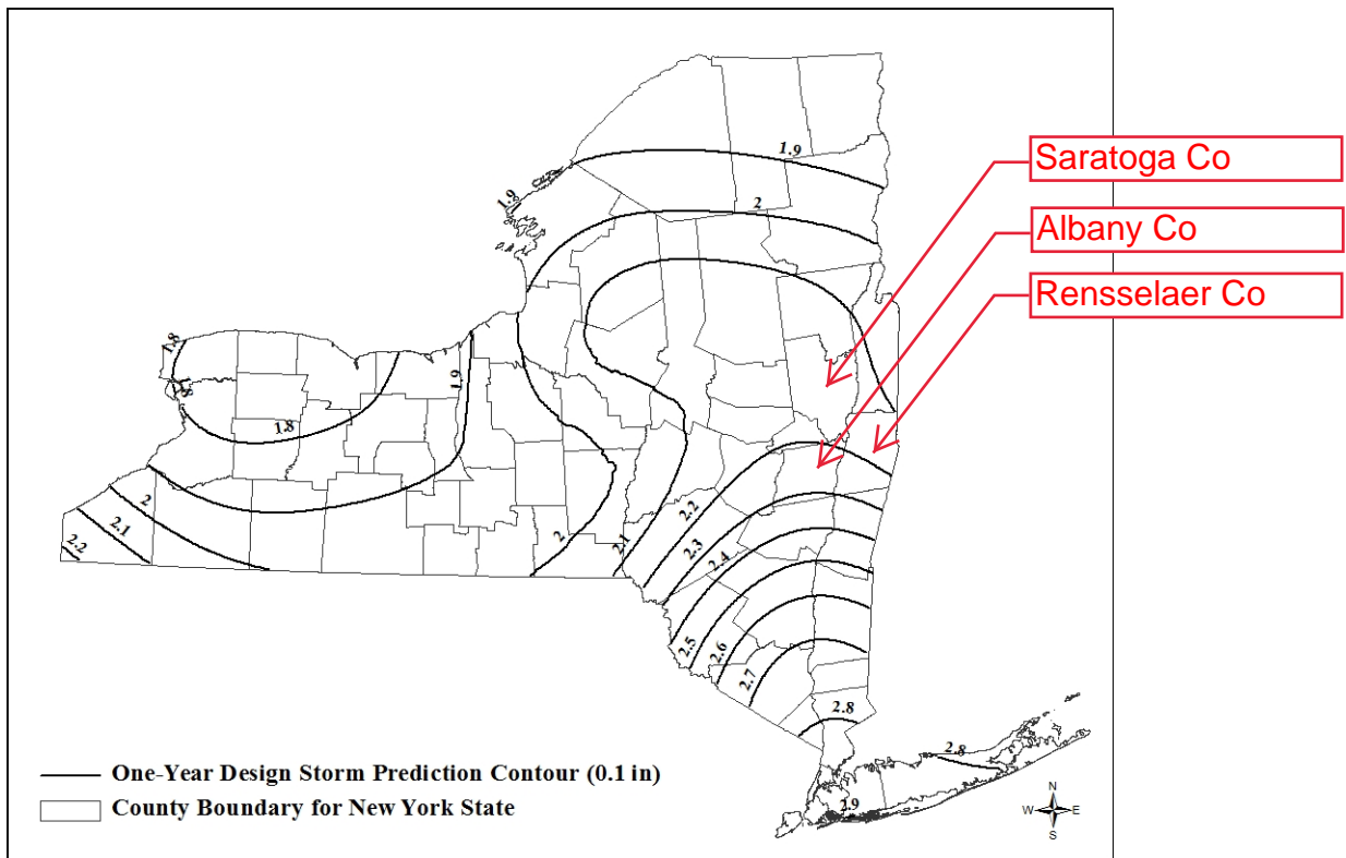
Figure 4.2: One-Year Design Storm in New York State (NYSDEC, 2013)
