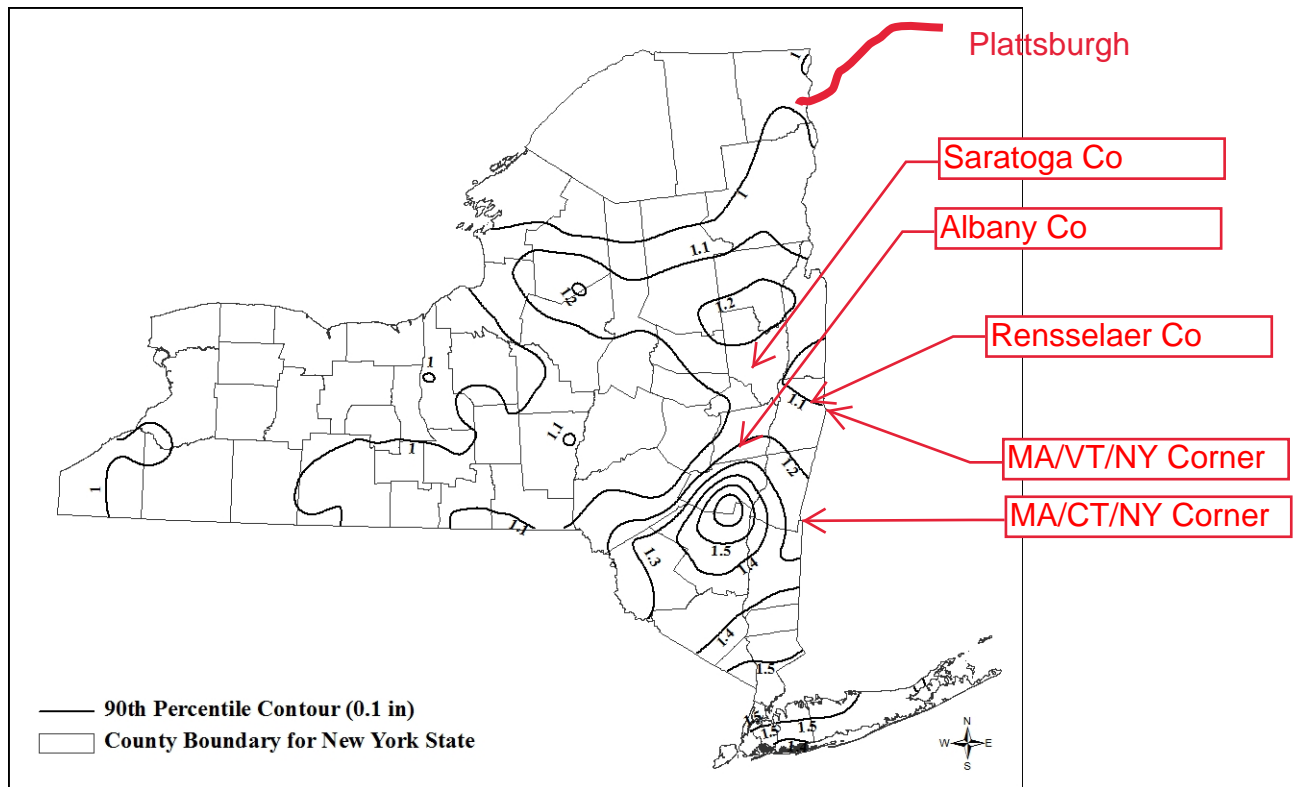
Figure 4.1: 90th Percentile Rainfall in New York State (NYSDEC, 2013)
