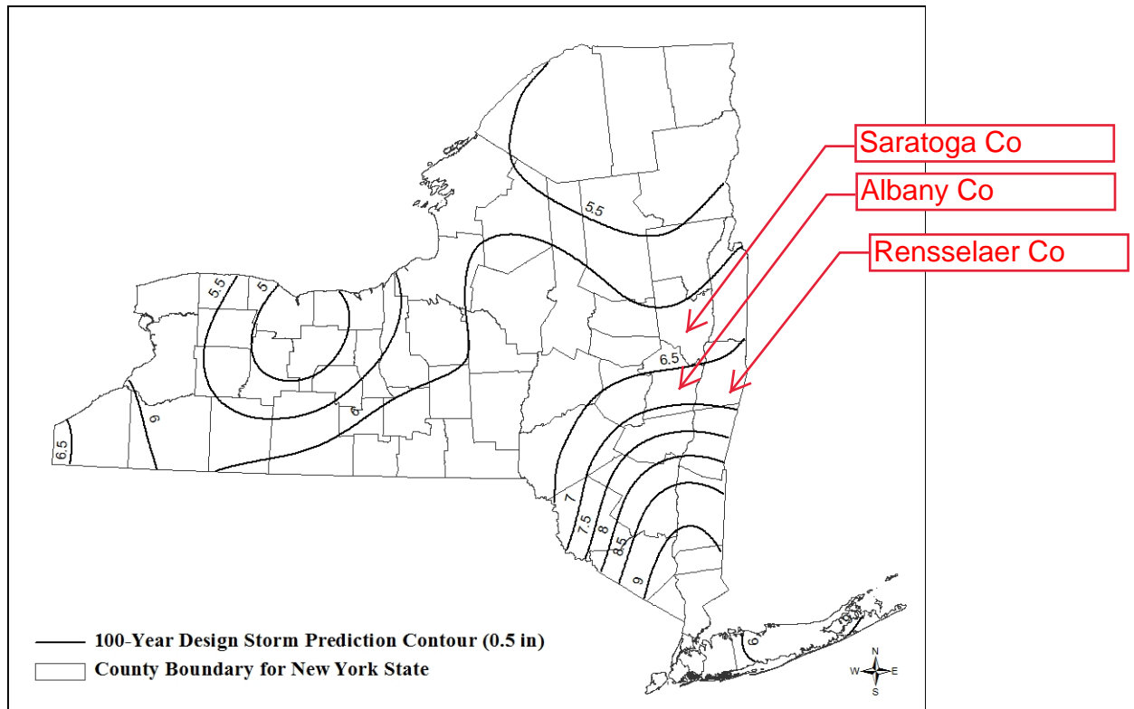
Figure 4.4: One Hundred-Year Design Storm in New York State (NYSDEC, 2013)
