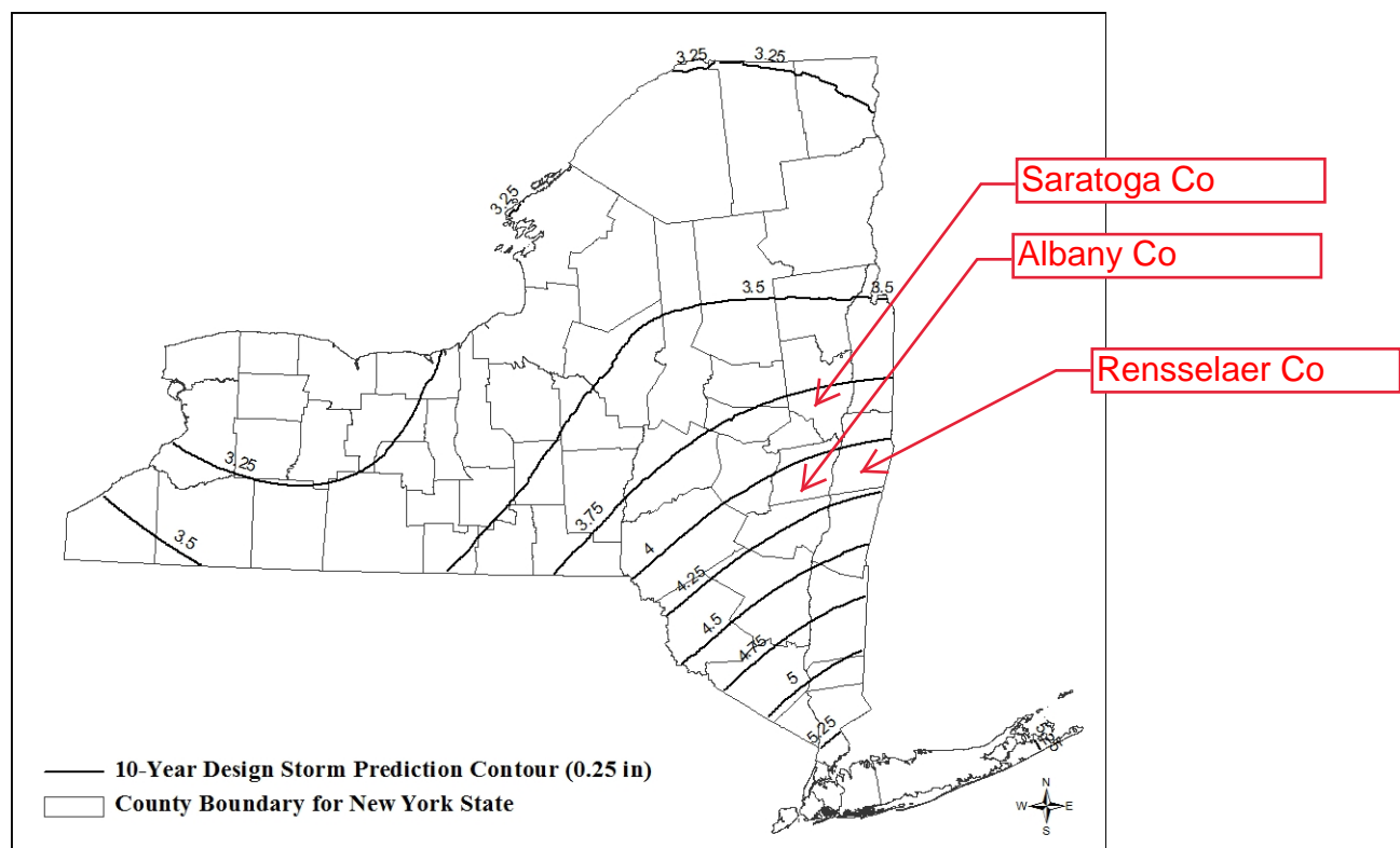
Figure 4.3: Ten-Year Design Storm in New York State (NYSDEC, 2013)
